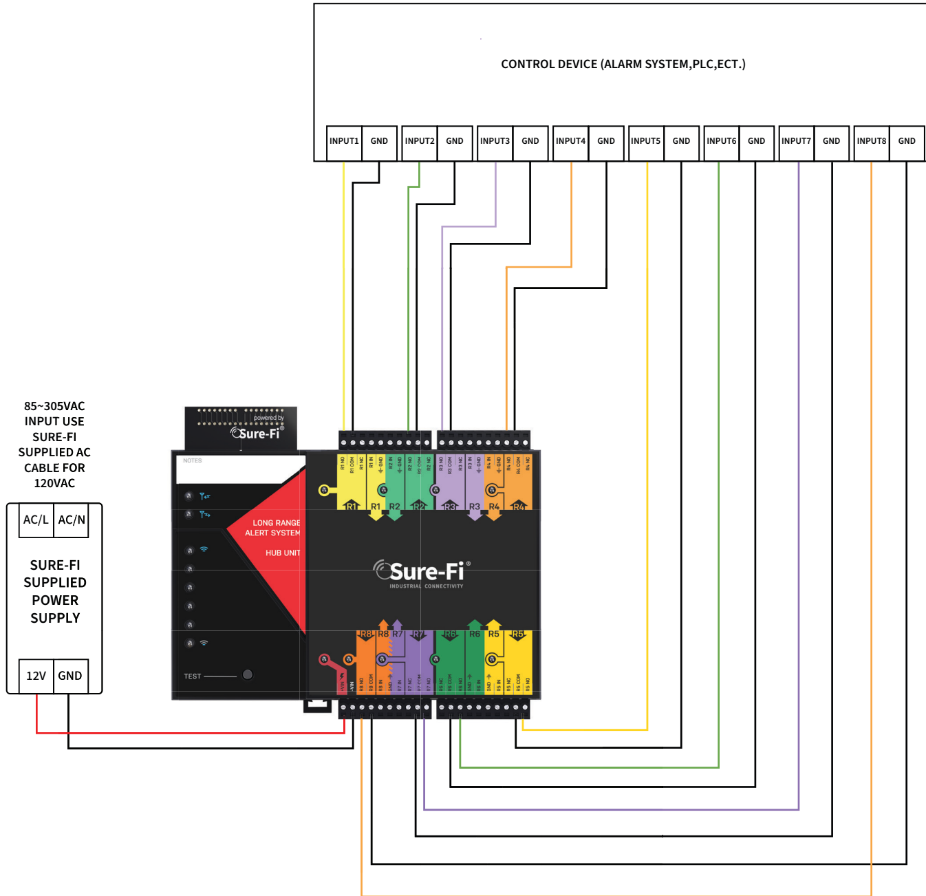
Typical wiring for 4:1 LRAS Hub using Sure-Fi supplied power supply and controller.
